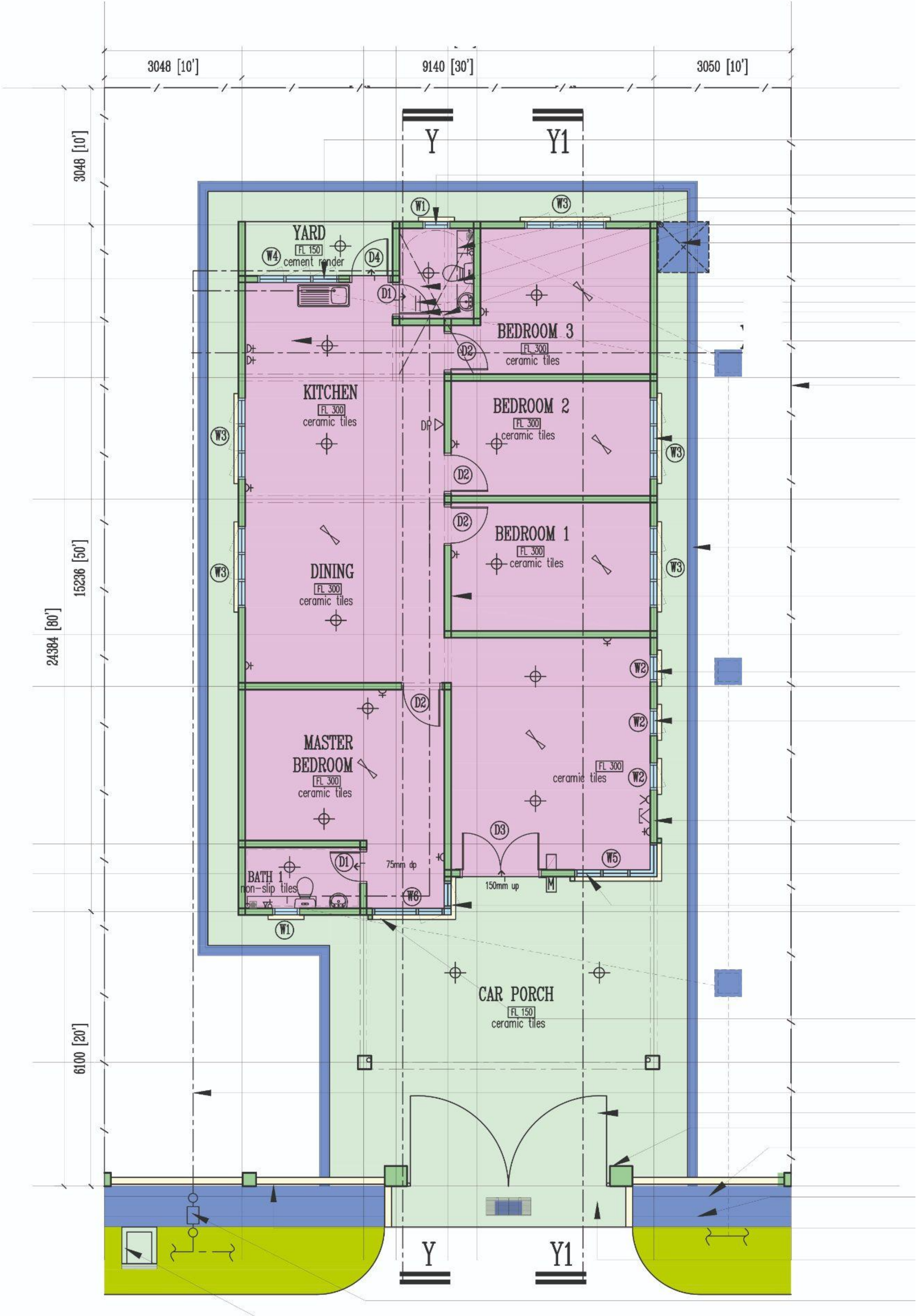
FLOOR PLAN
